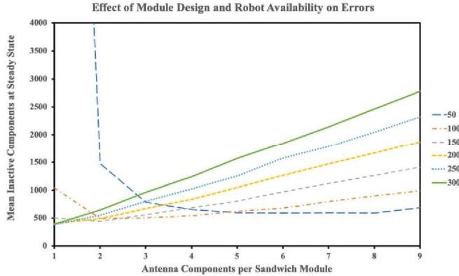
Figure 4. Graph of the effect of the number of components per sandwich module and the number of available robots on mean inactive components.
