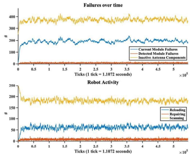
Figure 3. Graph of failures over time and robot activity over a simulation period of a week.
