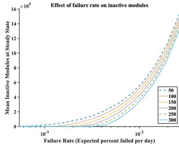
Figure 5 Graph of the effect of failure rate on mean inactive modules as a function of number of robots for a 950 m spaceteenna, at steady state
