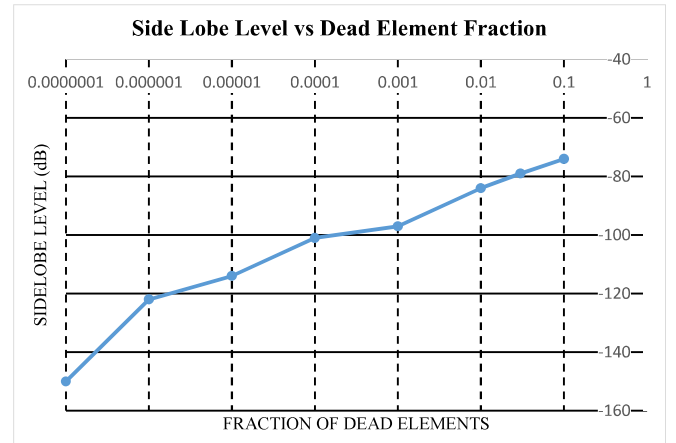
Figure 1. Loss of side lobe level reduction relative to main lobe versus fraction of dead elements randomly located 12 .
